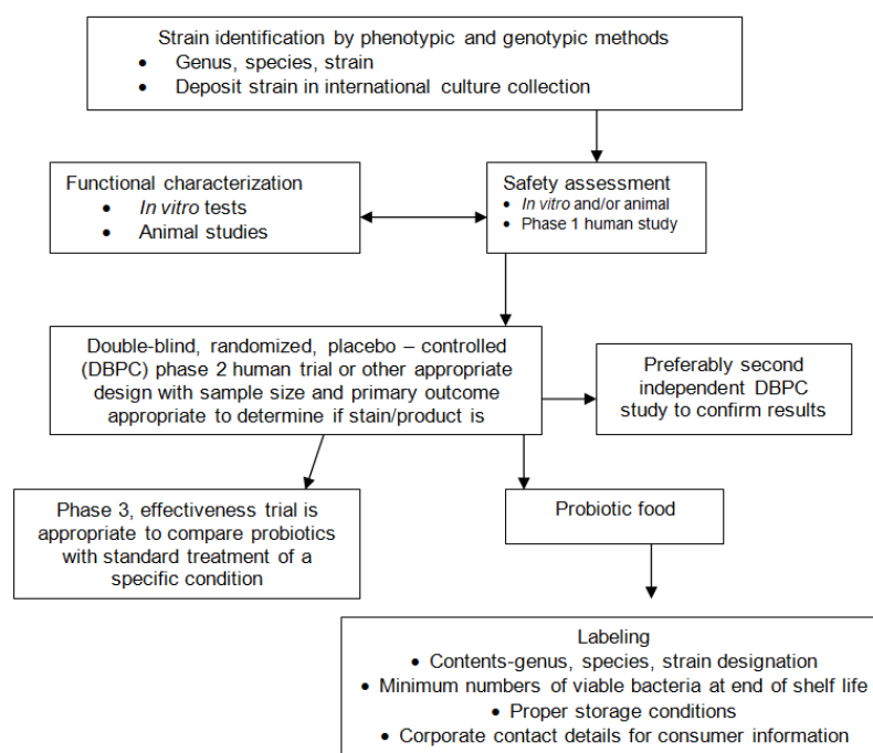
Figure 2: Assessment of probiotics. 24
